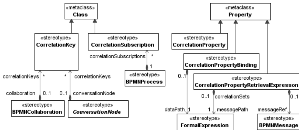
Figure 22: Correlation
