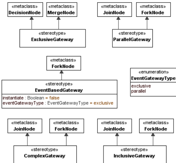
Figure 15: Gateways
