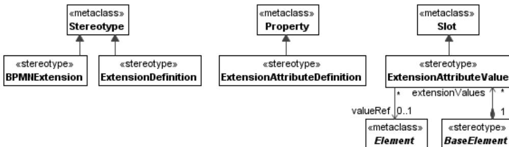
Figure 7: BPMN Extensions
