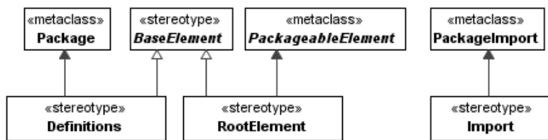
Figure 3: Definitions
