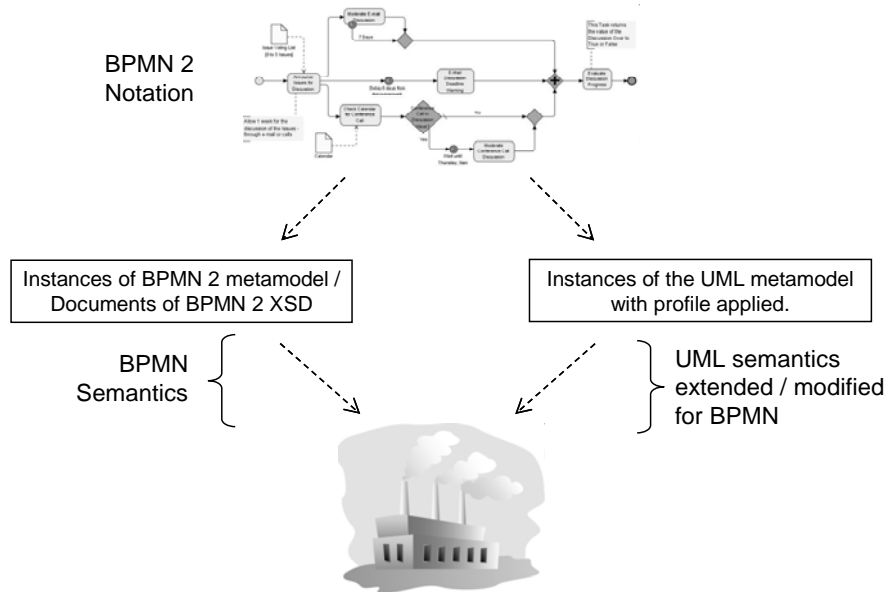
Figure 1: Equivalent Semantics
