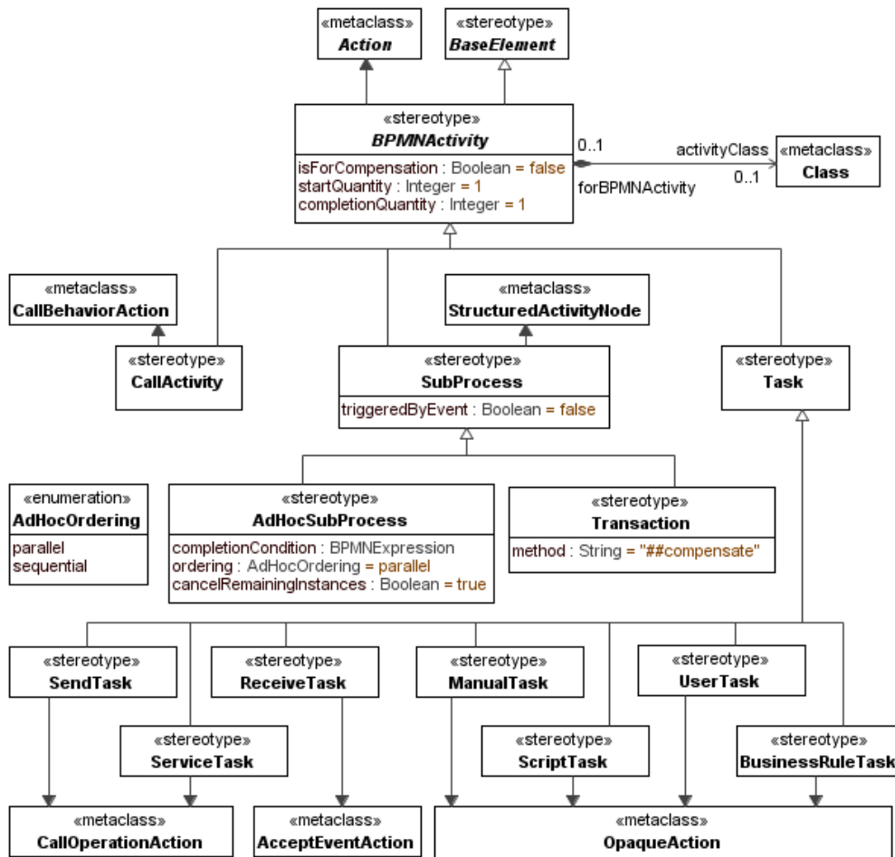
Figure 9: Activities
