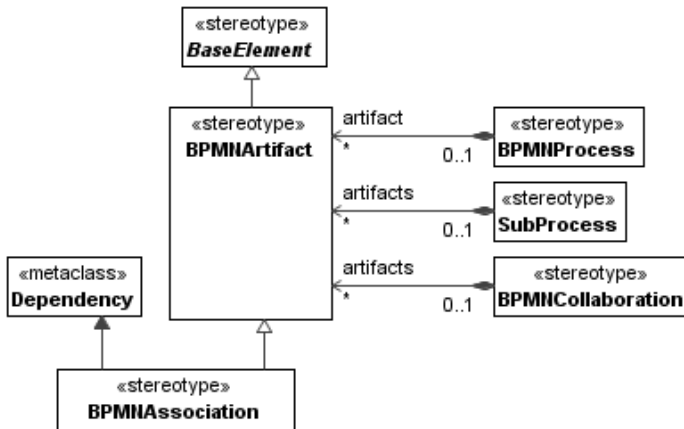
Figure 6: Artifacts
