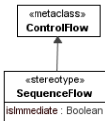
Figure 10: Sequence Flow
