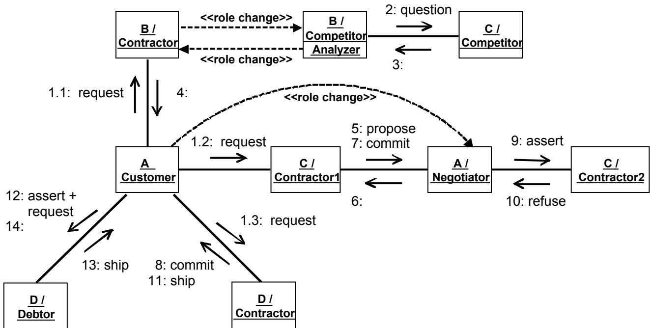
Figure 9. An example of a collaboration diagram depicting an interaction among agents playing multiple roles.
