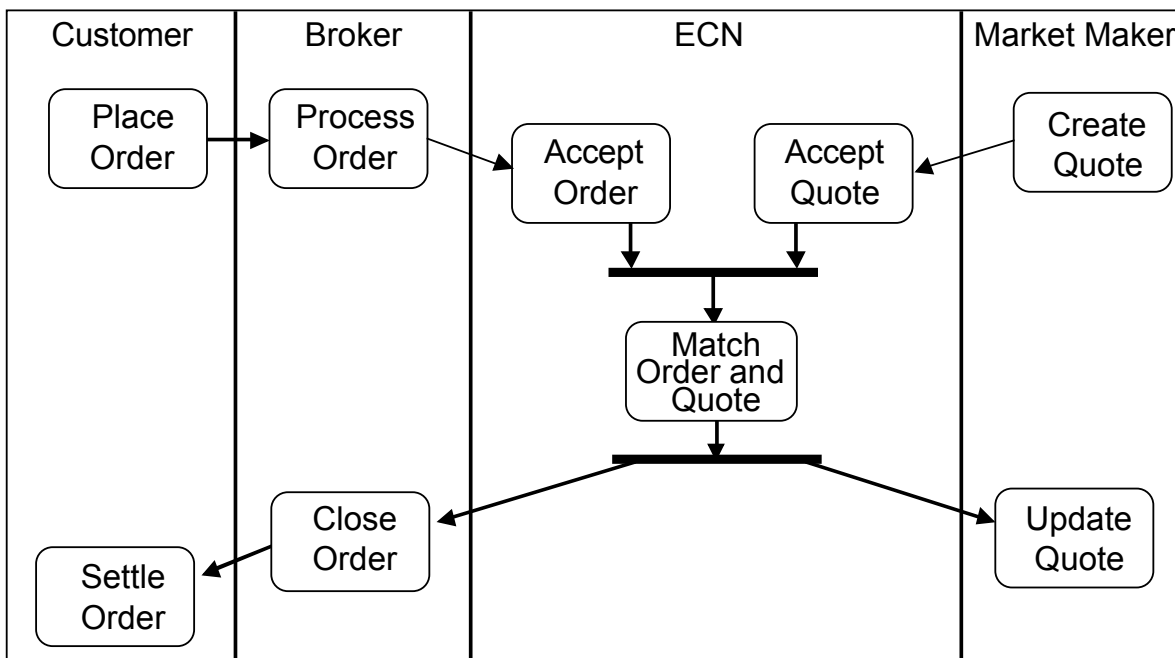
Figure 11. An activity diagram that depicts a stock sale protocol among several agents.
