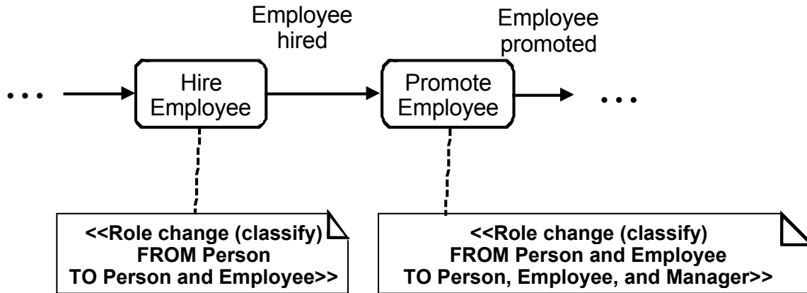
Figure 21. Dynamic classification (role changes) expressed as notes.
