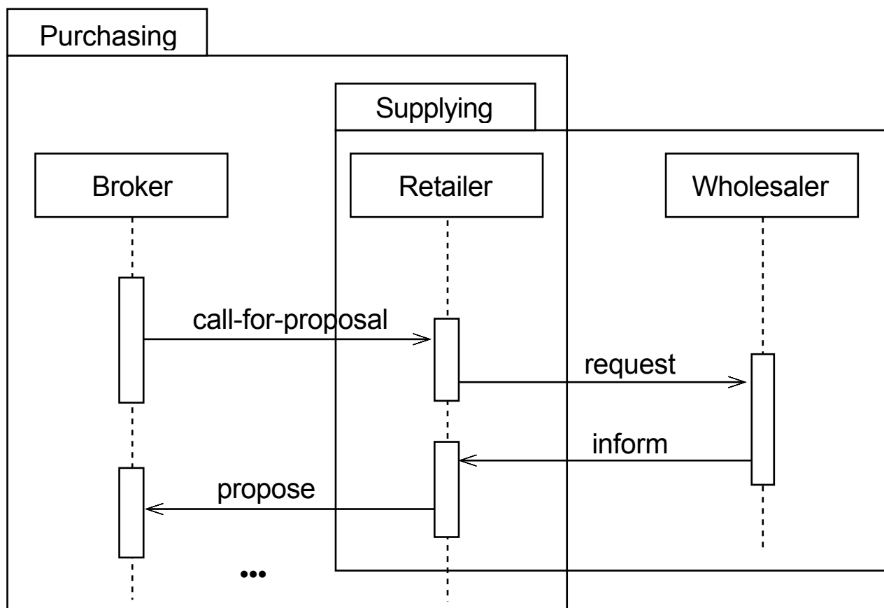
Figure 3. Using packages to express nested protocols.
