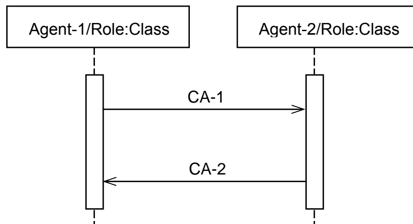
Figure 6 Basic format for agent communication.
