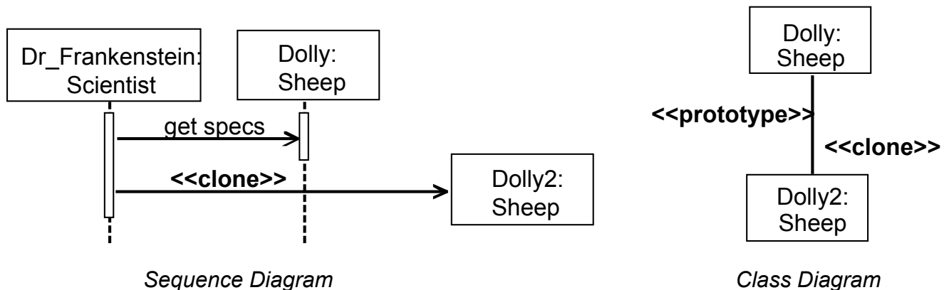
Figure 24. Representing cloning using sequence and class diagrams.
