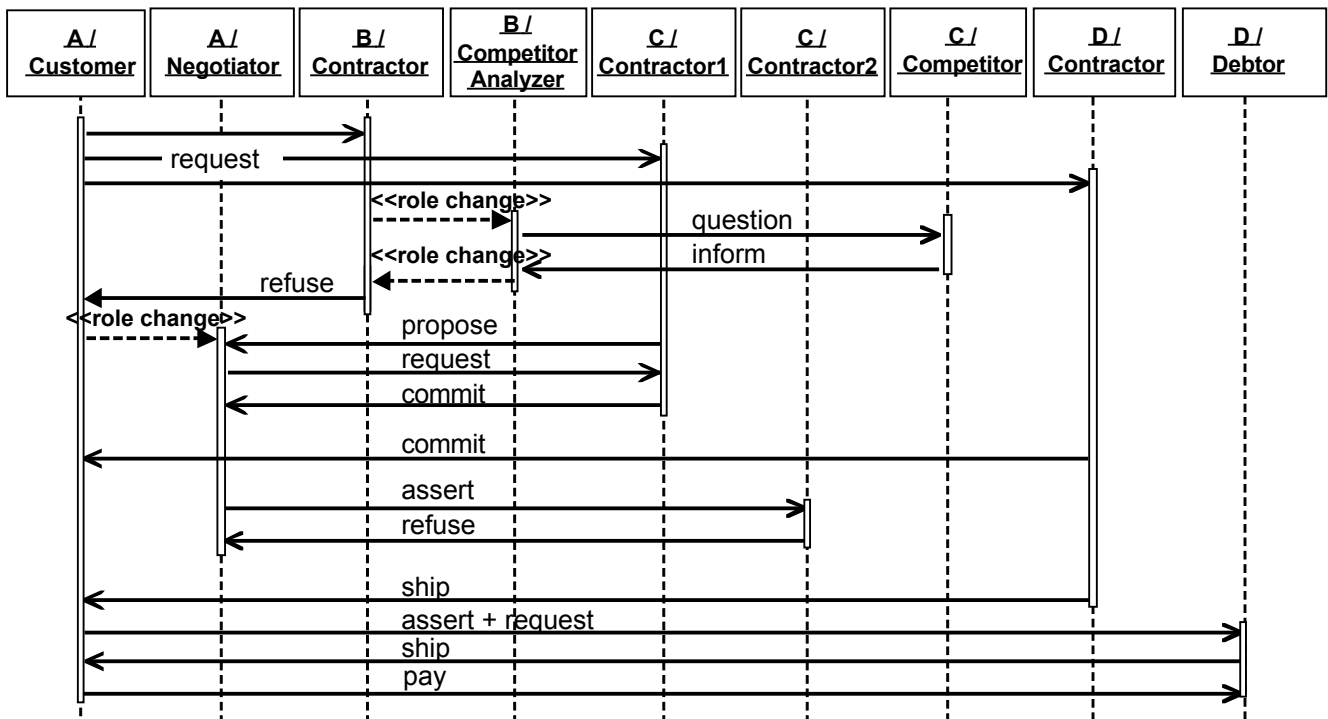
Figure 10. A sequence diagram version of Fig. 9.
