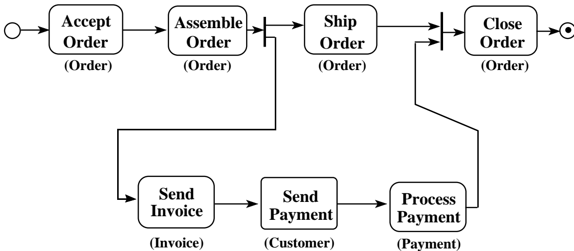
Figure 20. An activity diagram with activities labeled with the appropriate agent role.
