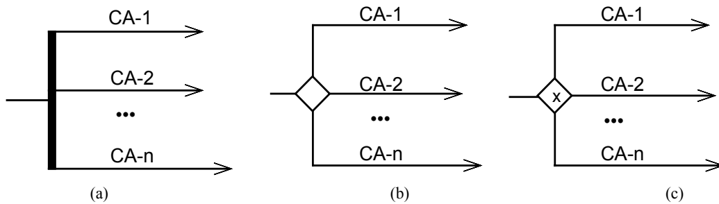
Figure 7. Some recommended extensions that support concurrent threads of interaction.
