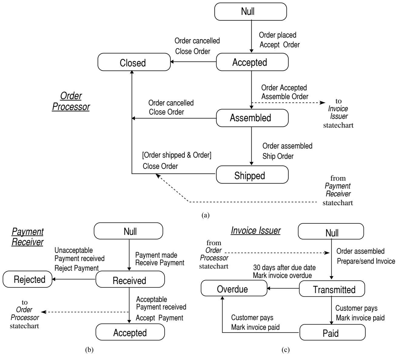
Figure 14. Statechart that specifies order processing behavior for the three agents.
