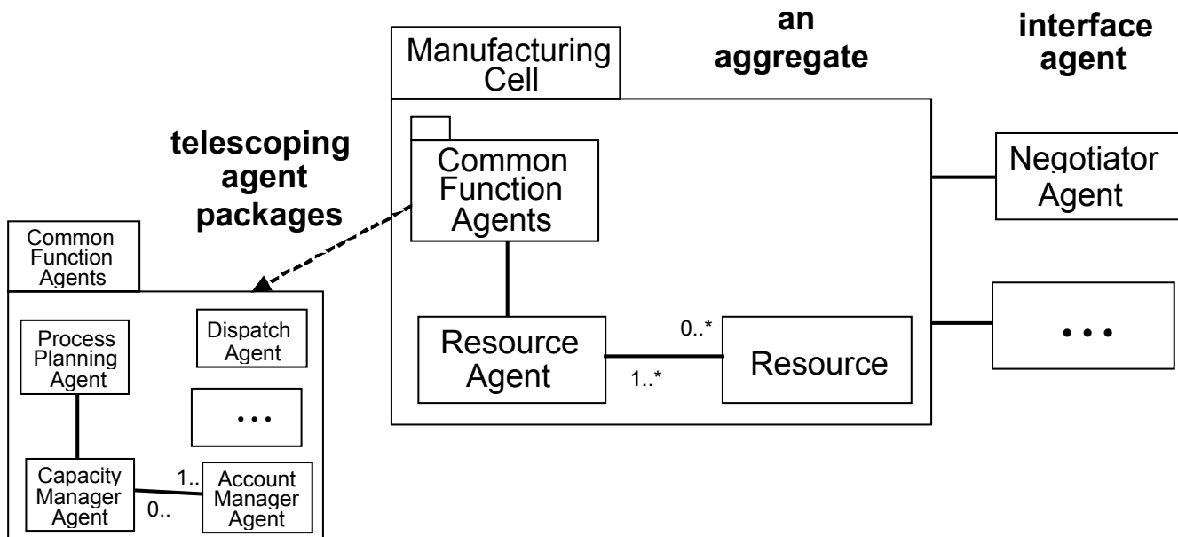
Figure 22. Package specifying agents instead of operations as interface points.
