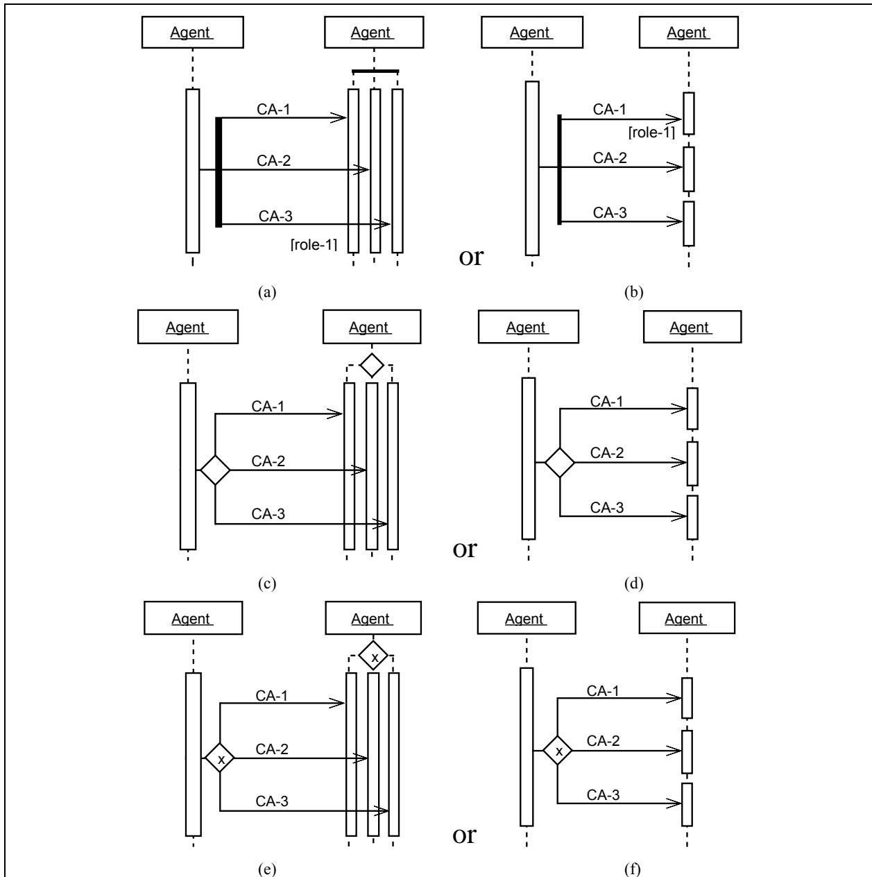
Figure 8. Multiple techniques to express concurrent communication with an agent playing multiple roles or responding to different CAs.
