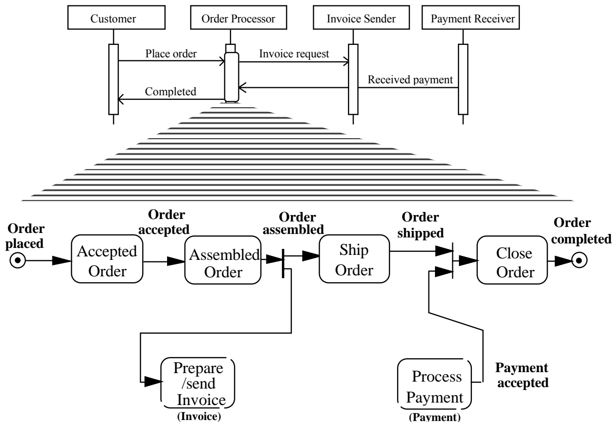
Figure 13. An activity diagram that specifies order processing behavior for an Order agent.
