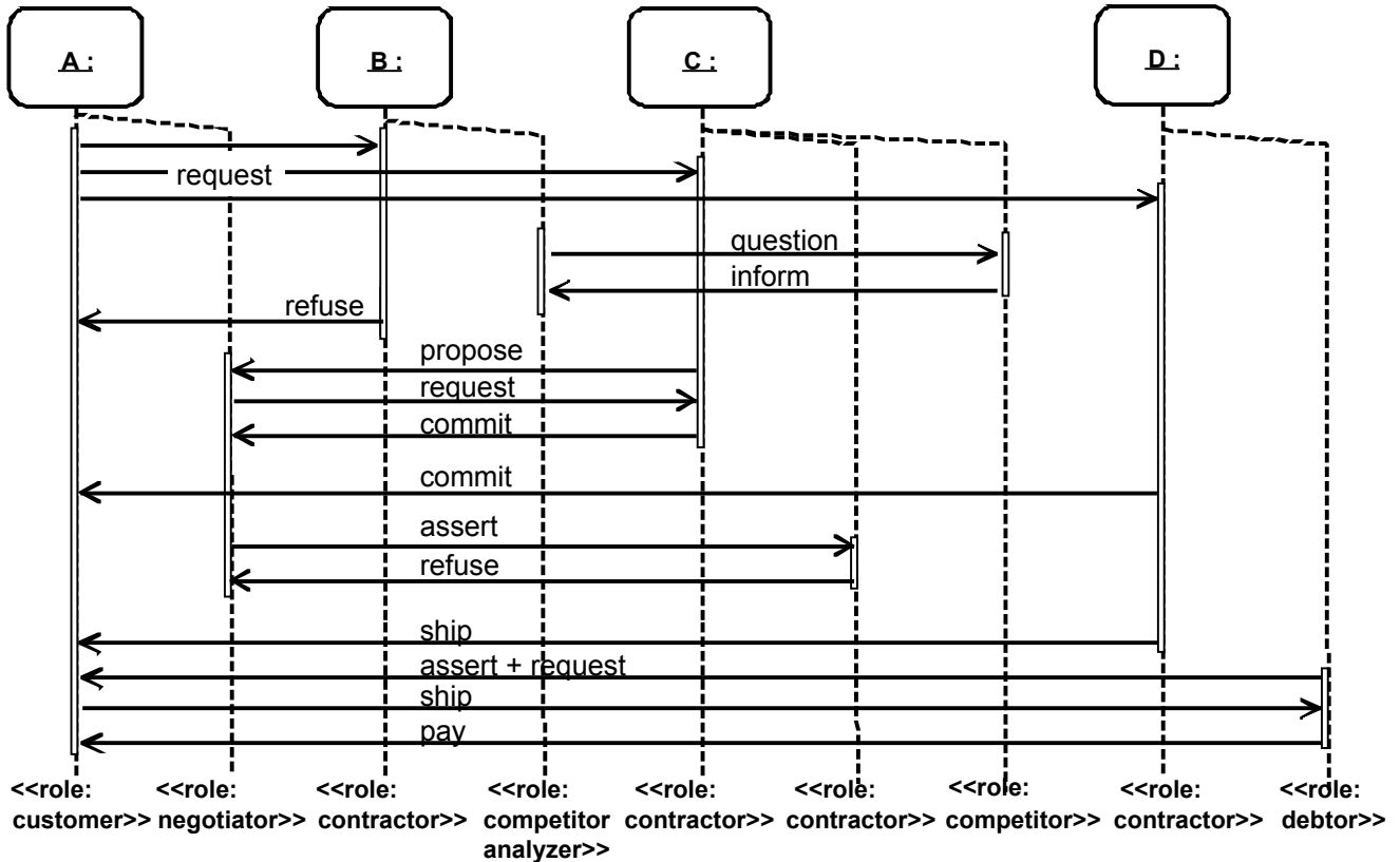
Figure 16. Role modeling representing each role with its own lifeline.
