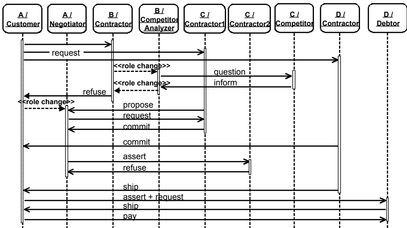
Figure 15. Role modeling using the existing UML 1.3 "slash" notation.
